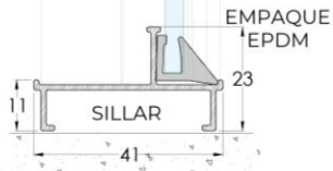
4 CORTE VERTICAL SILLAR
